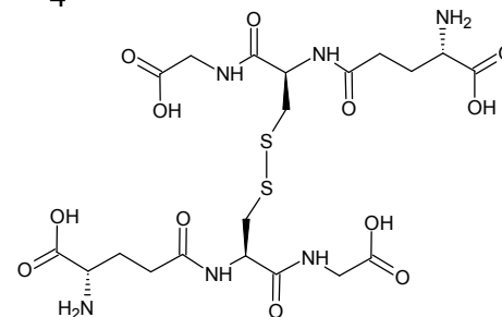
Glutathione disulfide
