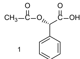
(+)-O-Acetyl-L-mandelic Acid
