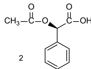
(-)-O-Acetyl-D-mandelic Acid
