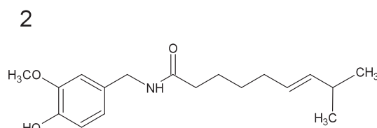
Capsaicin (MW 305.4)
