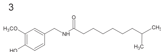
Dihydrocapsaicin (MW 307.4)
