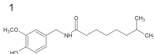
Nordihydrocapsaicin (MW 293.4)
