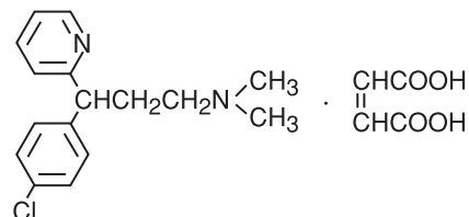
Chlorpheniramine maleate
