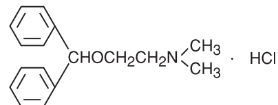
Diphenhydramine hydrochloride
